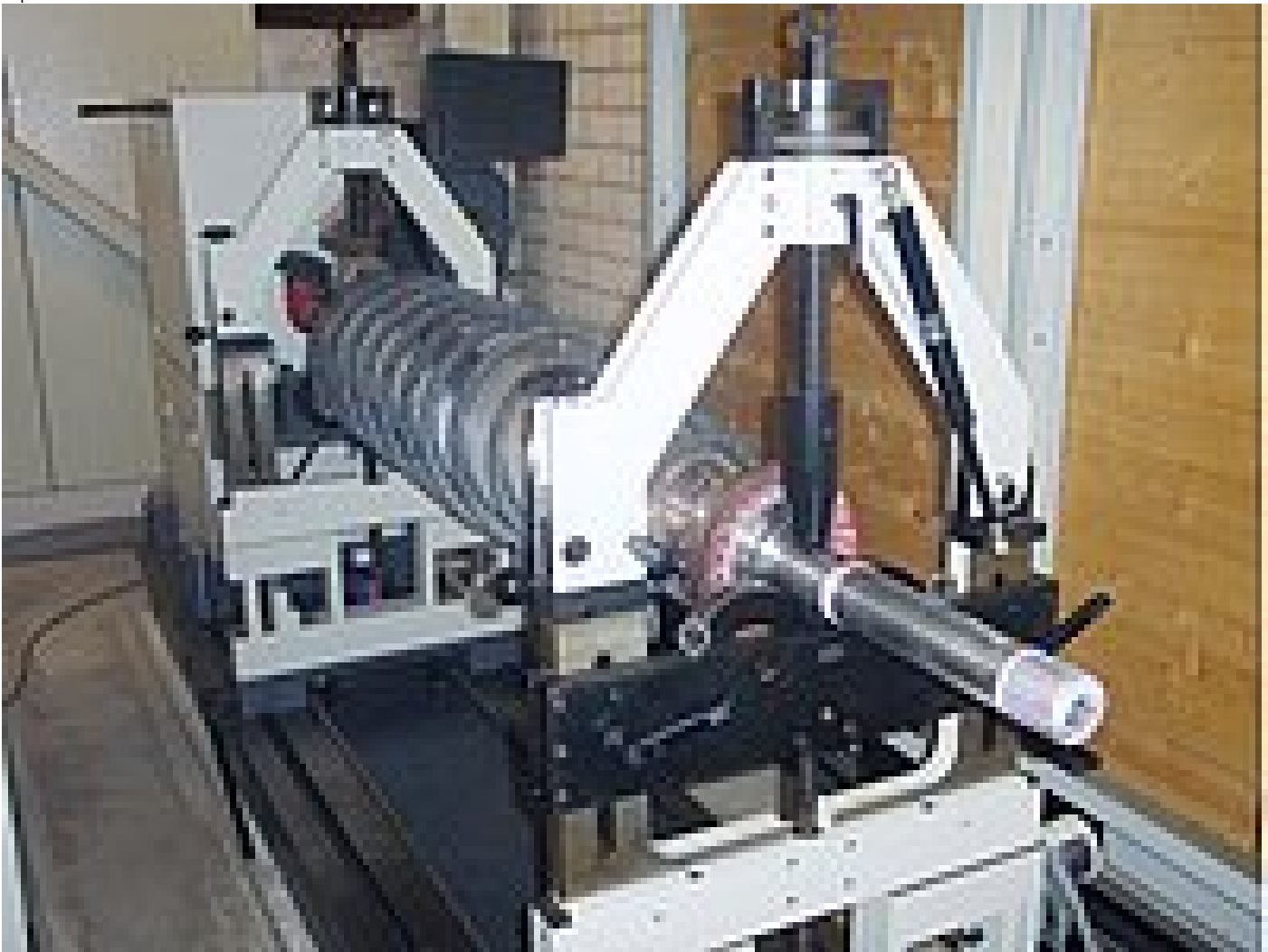
Centrifuge rotor on the balancing stand
